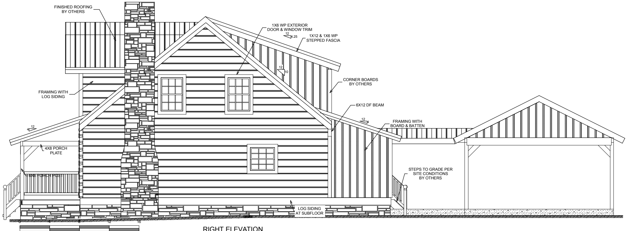
RIGHT ELEVATION NOTE: GRADE CONDITIONS TO BE VERIFIED ON SITE
